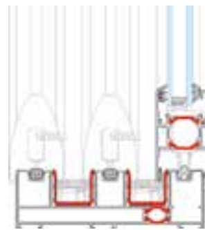
Notus tri-rail
