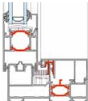
Notus mono-rail
