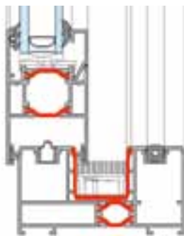
Notus duo-rail
